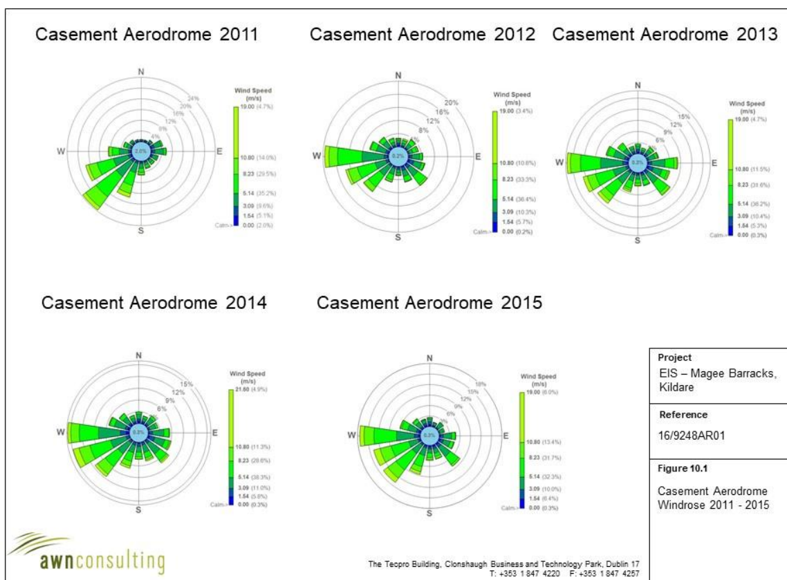
Fig. 10.1: Casement Aerodrome windrose 2011 - 2015
